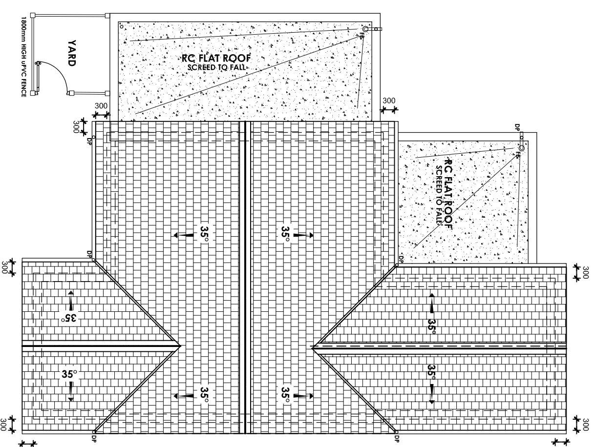
ROOF PLAN 1:100
