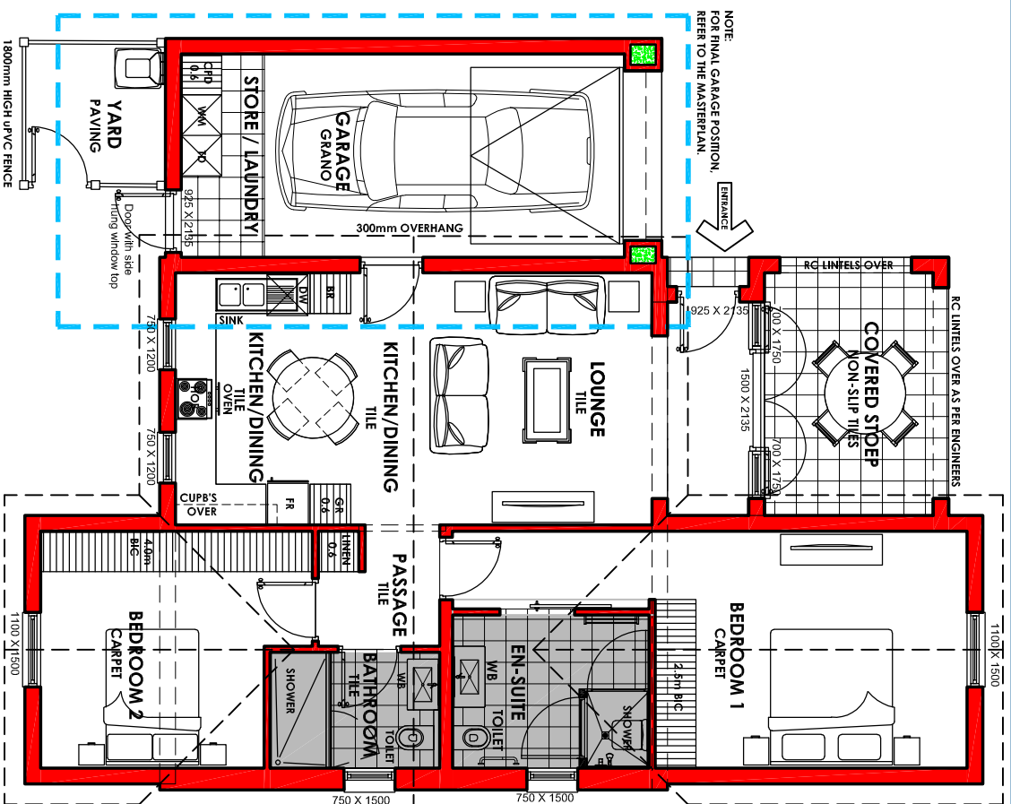
FLOOR PLAN 1:100
