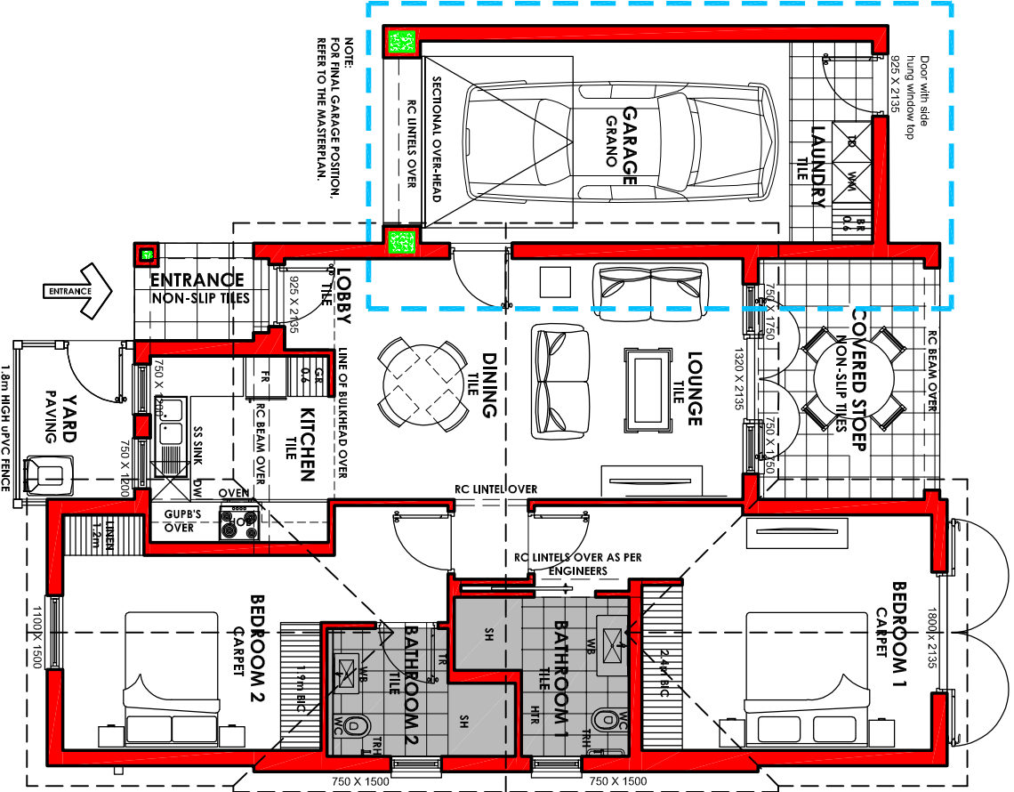
FLOOR PLAN 1:100
