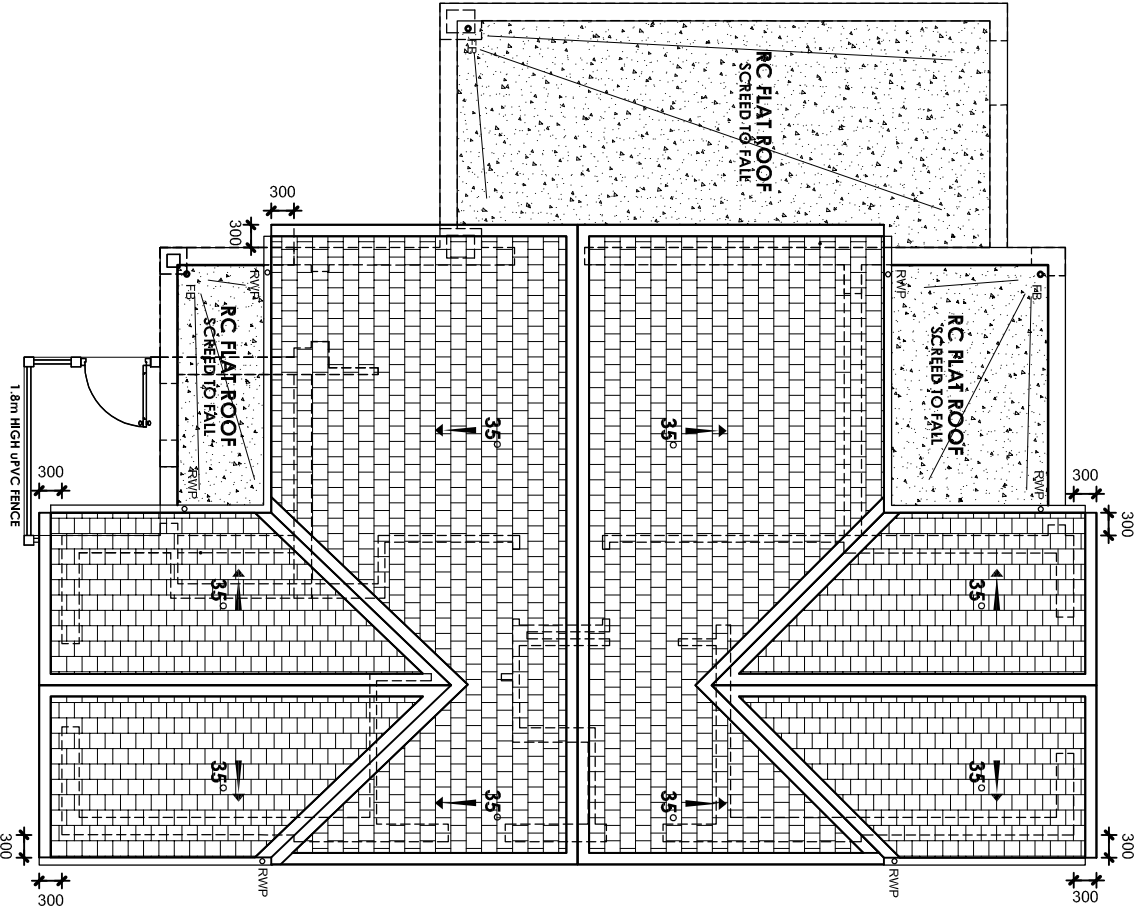
ROOF PLAN 1:100
