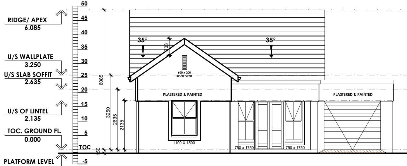
FRONT ELEVATION 1:100
