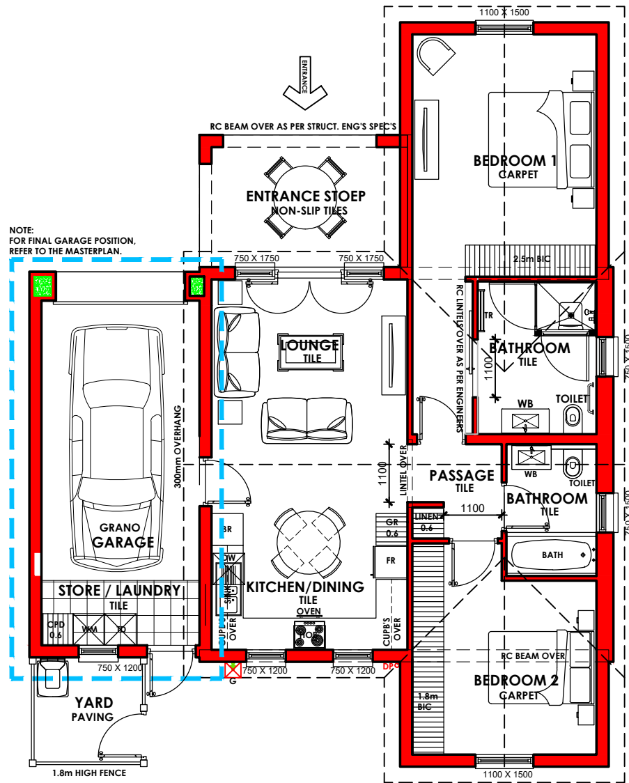
FLOOR PLAN 1:100
