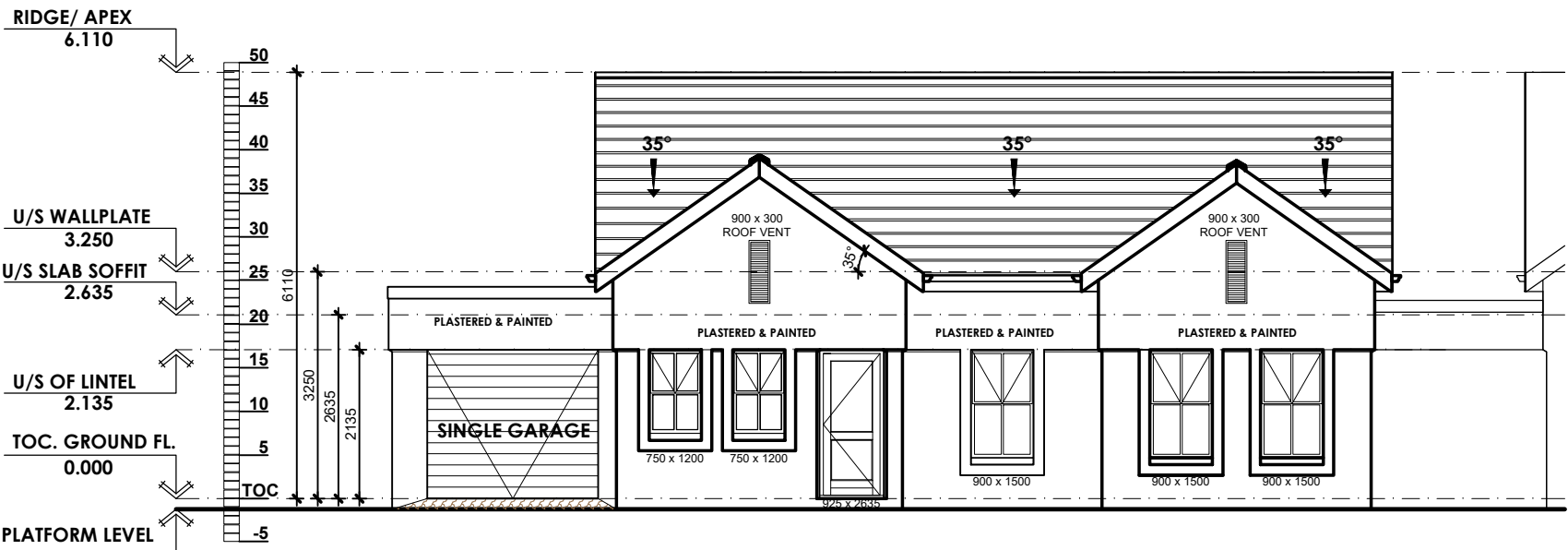
FRONT ELEVATION 1:100
