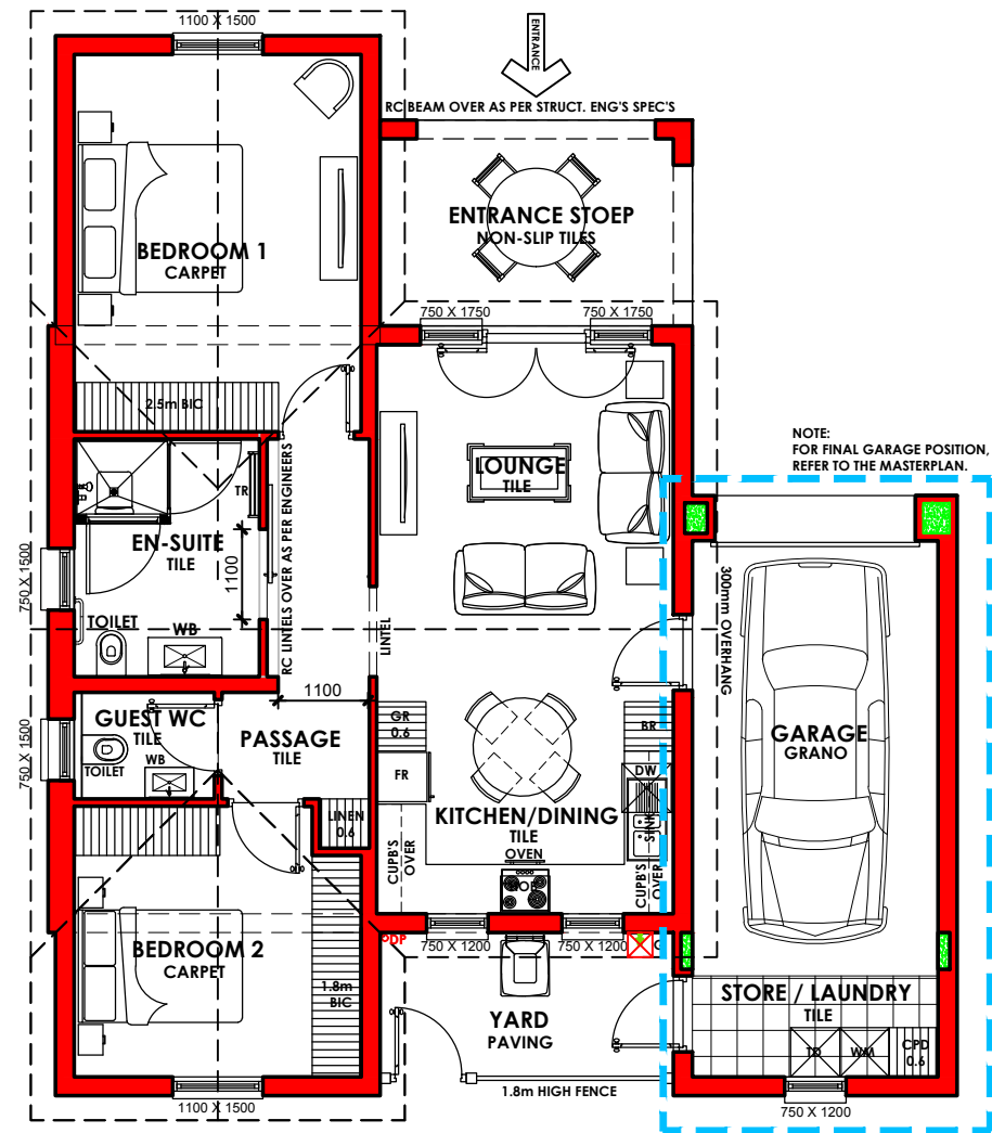
FLOOR PLAN 1:100
