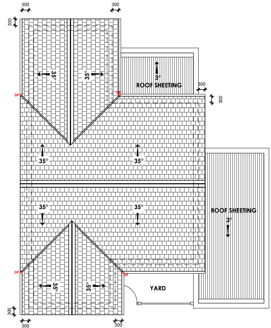
ROOF PLAN 1:100
